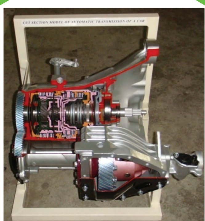
Cutsection Model Of Automatic Transition Of A Car
