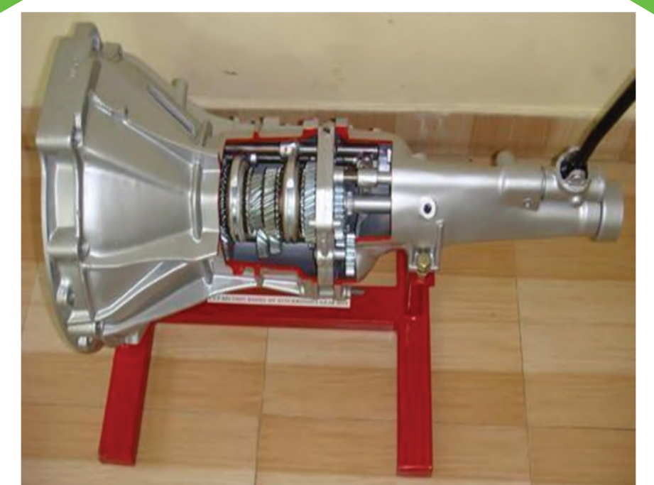
Gear Box Cut Section
